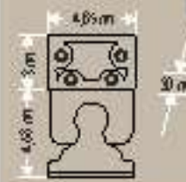
CT-4697 WALL WASHER
